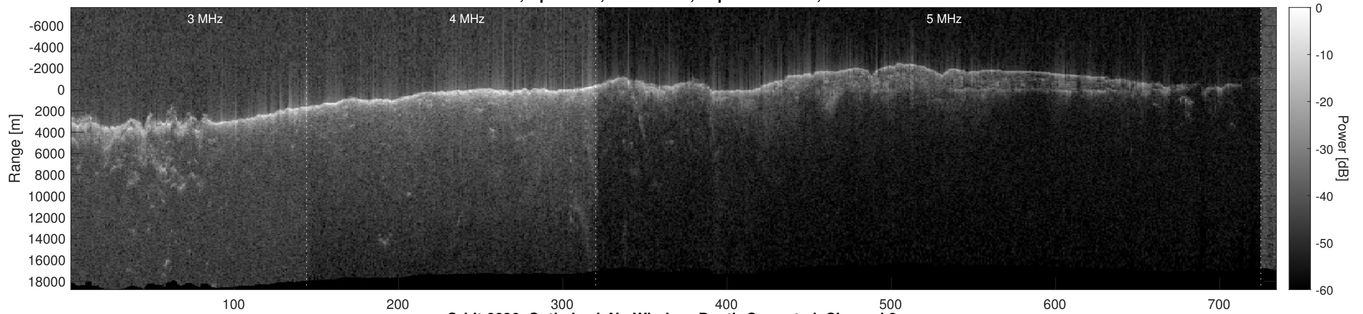
Orbit 6636, Optimized, No Window, Depth-Corrected, Channel 2
