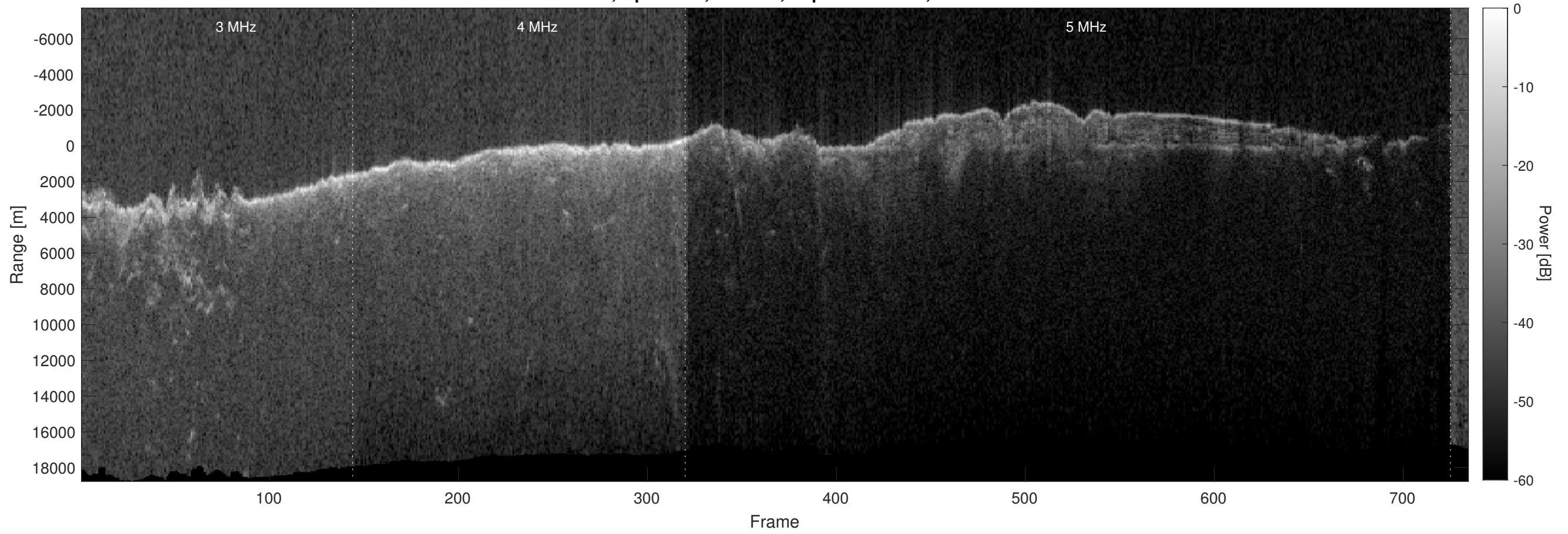
Orbit 6636, Optimized, Window, Depth-Corrected, Channel 2
