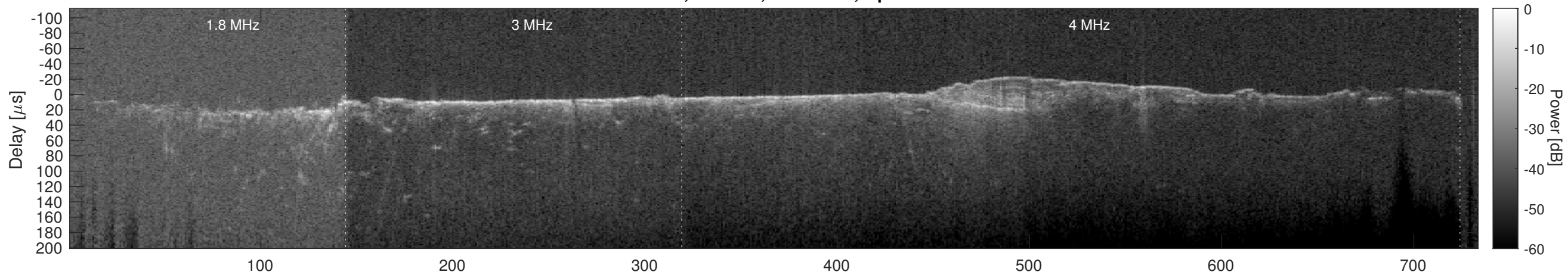
Orbit 6637, Cluttergram
