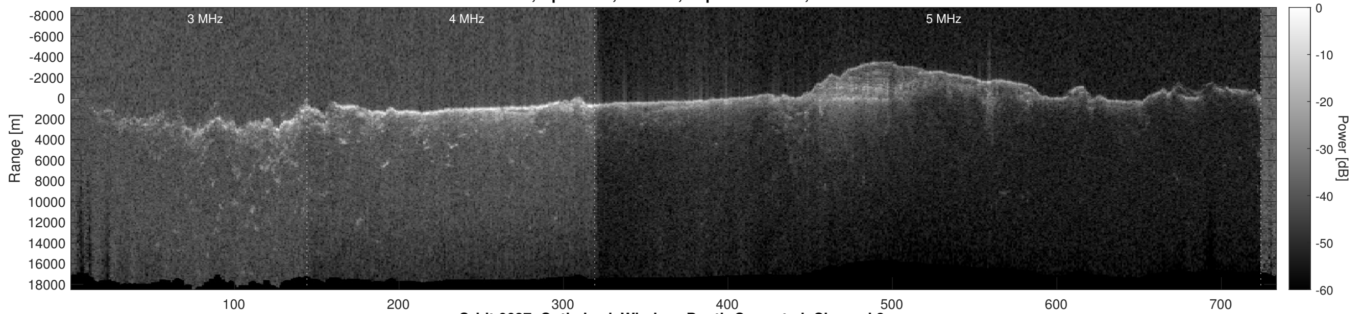
Orbit 6637, Optimized, Window, Depth-Corrected, Channel 2
