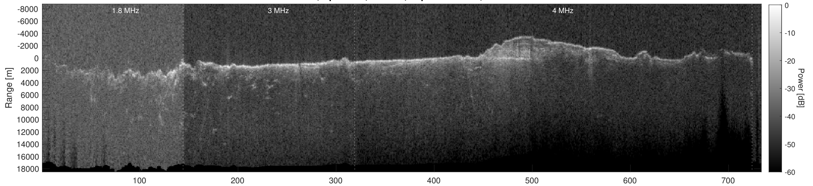
Orbit 6637, Depth-Corrected Cluttergram
