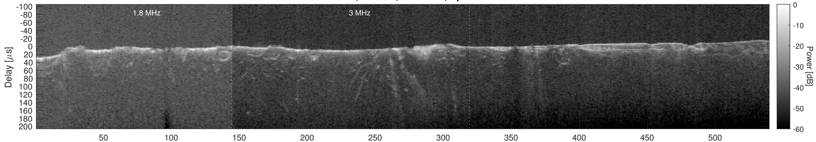
Orbit 6638, Cluttergram
