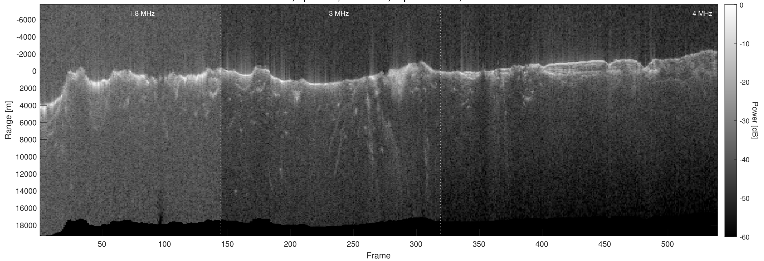
Orbit 6638, Optimized, No Window, Depth-Corrected, Channel 2
