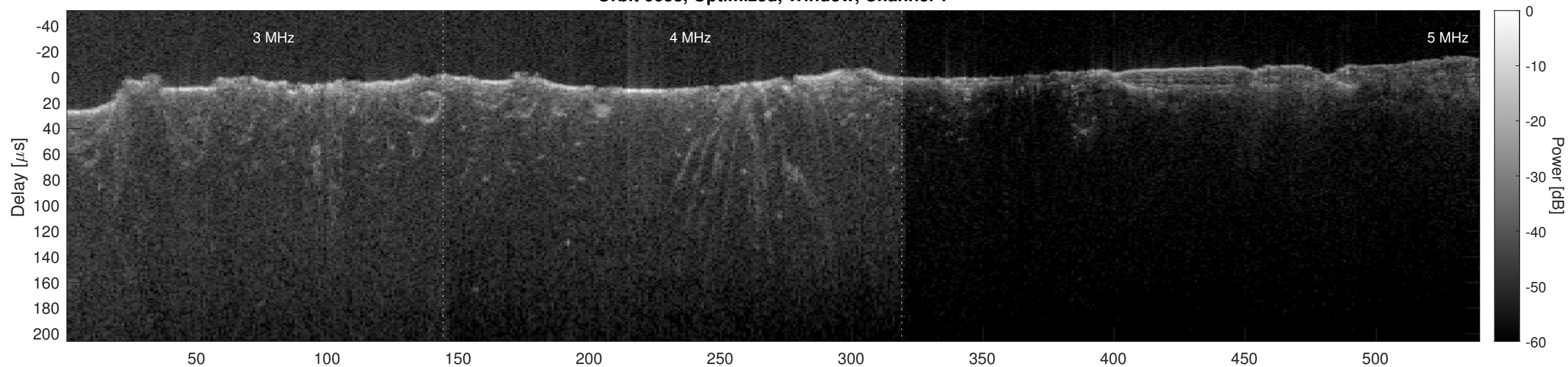
Orbit 6638, Optimized, Window, Channel 2
