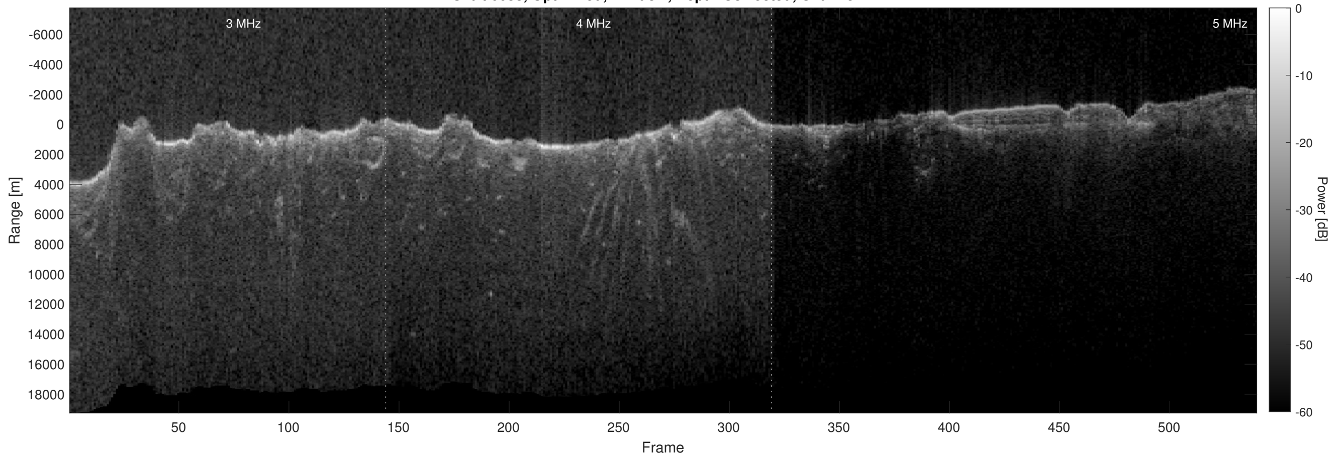
Orbit 6638, Optimized, Window, Depth-Corrected, Channel 2
