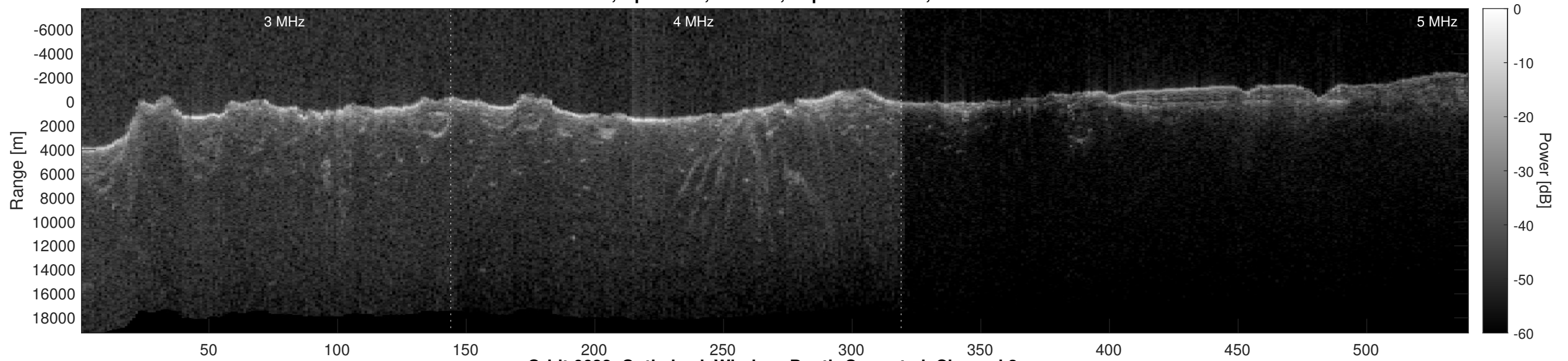
Orbit 6638, Optimized, Window, Depth-Corrected, Channel 2
