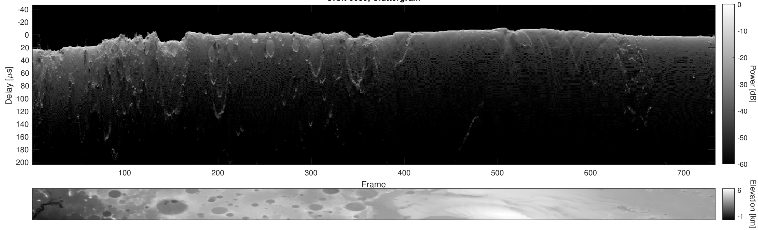
Orbit 6639, Cluttergram
