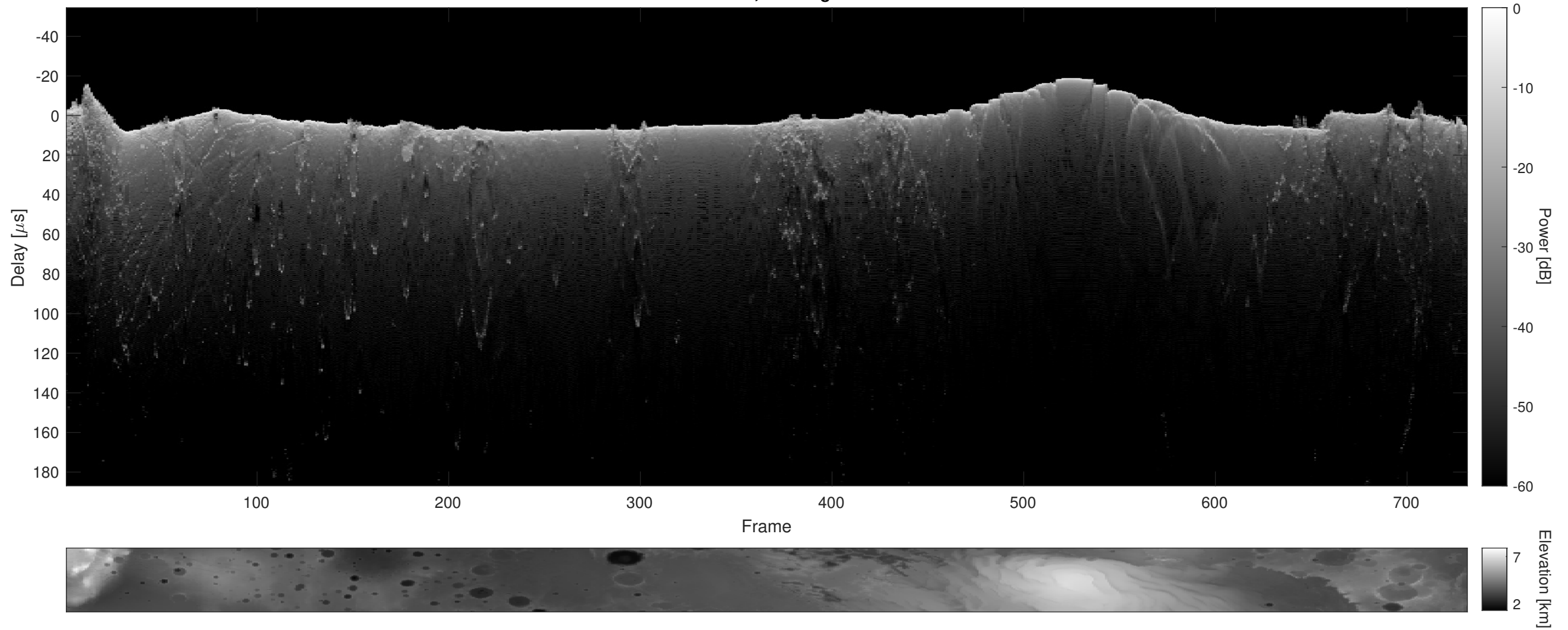
Orbit 6641, Cluttergram
