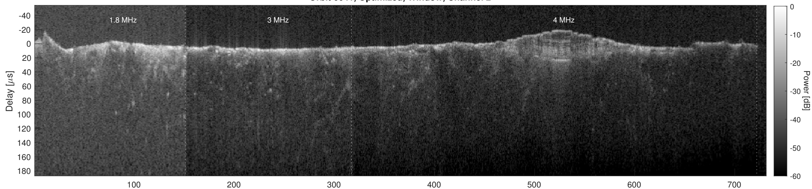
Orbit 6641, Cluttergram
