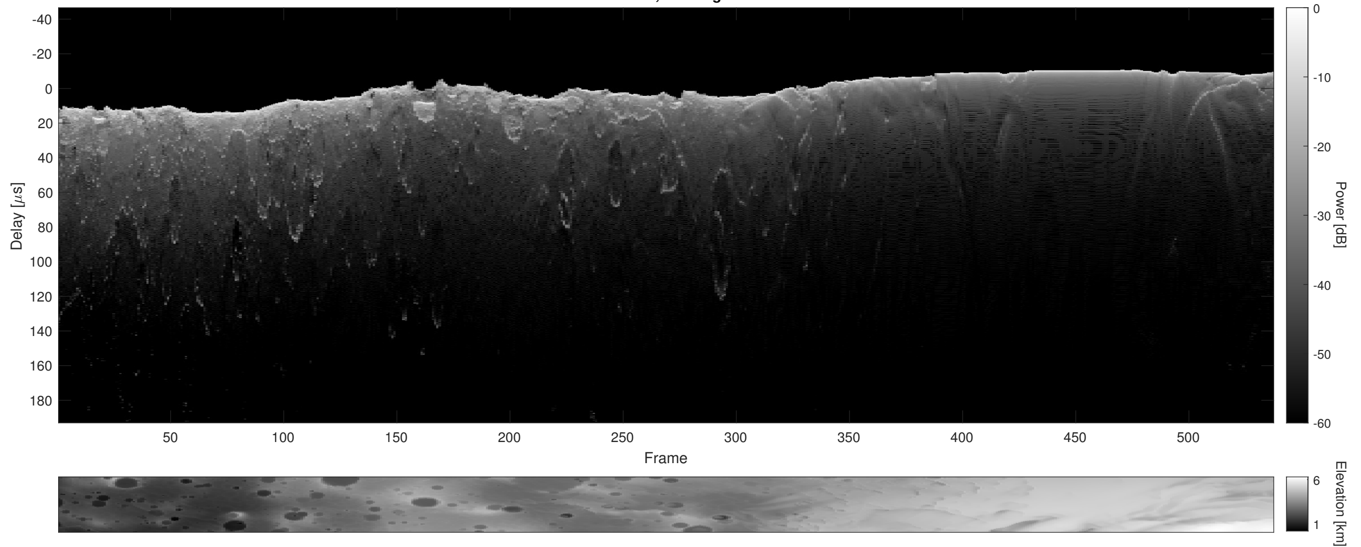
Orbit 6642, Cluttergram
