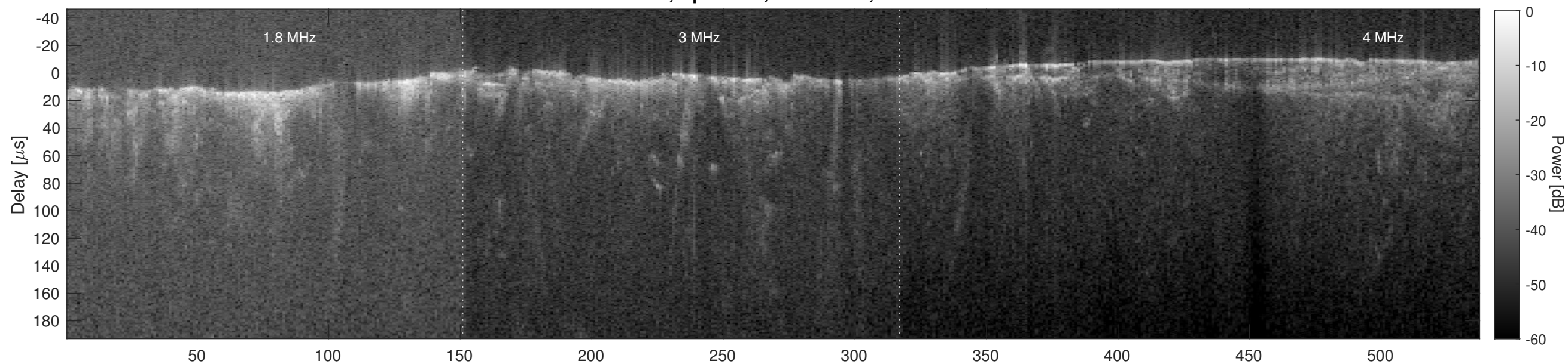
Orbit 6642, Cluttergram
