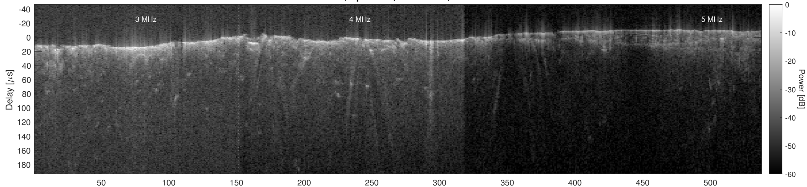
Orbit 6642, Optimized, No Window, Channel 2
