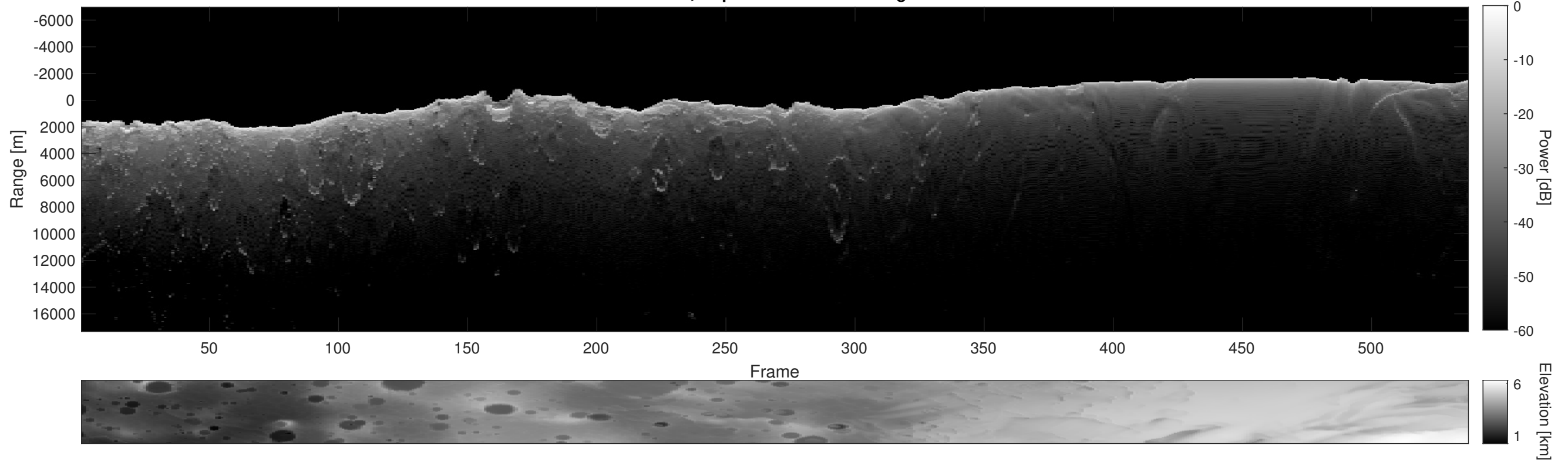
Orbit 6642, Depth-Corrected Cluttergram
