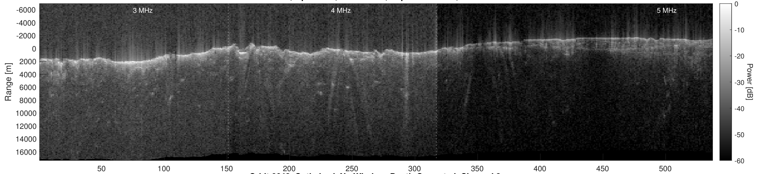
Orbit 6642, Optimized, No Window, Depth-Corrected, Channel 2
