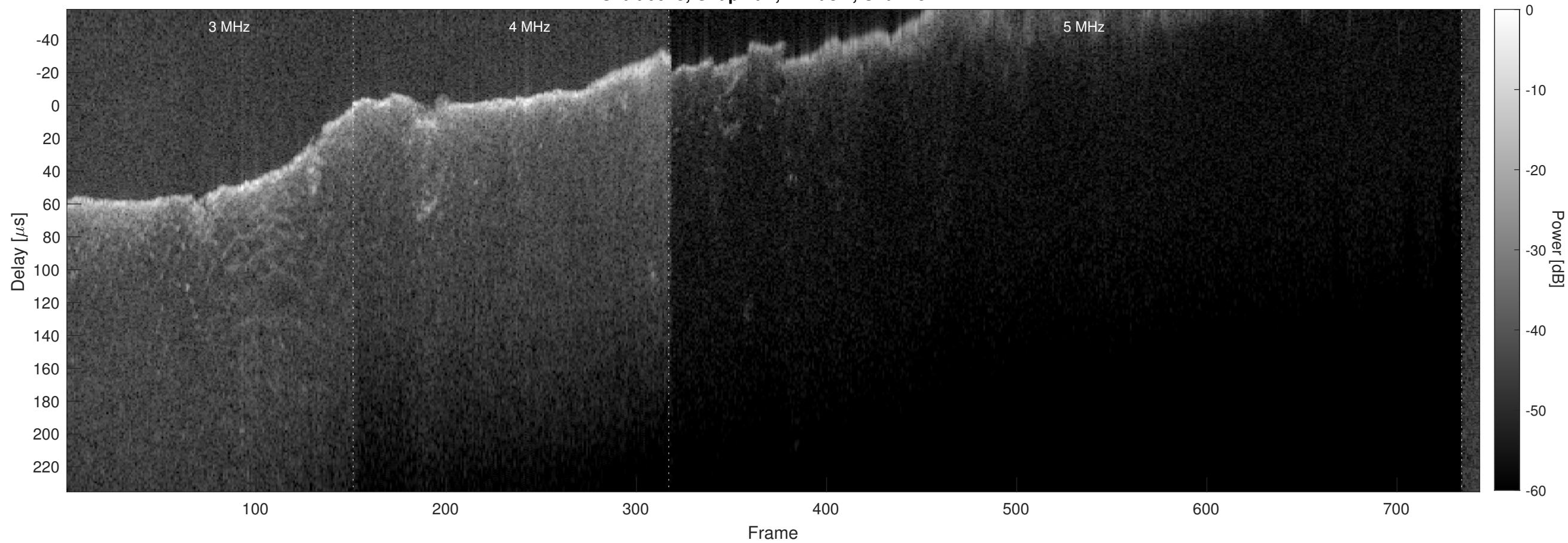
Orbit 6643, Chapman, Window, Channel 2
