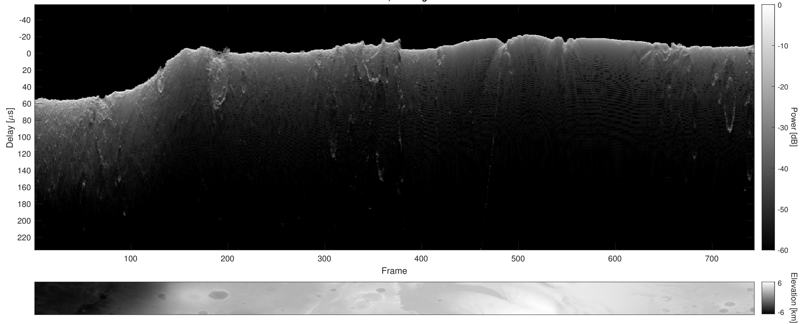
Orbit 6643, Cluttergram
