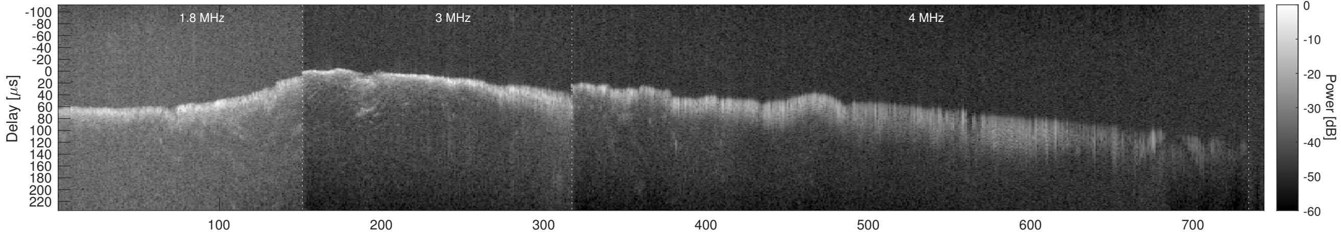
Orbit 6643, Window, Channel 2, Chapman
