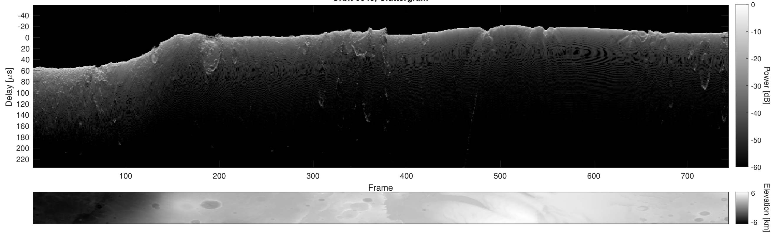
Orbit 6643, Cluttergram
