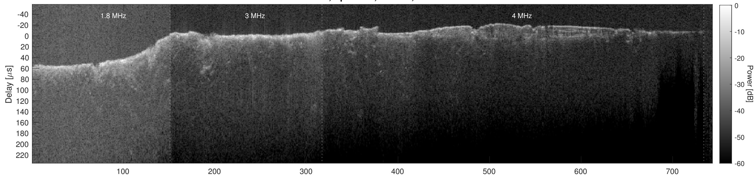
Orbit 6643, Cluttergram
