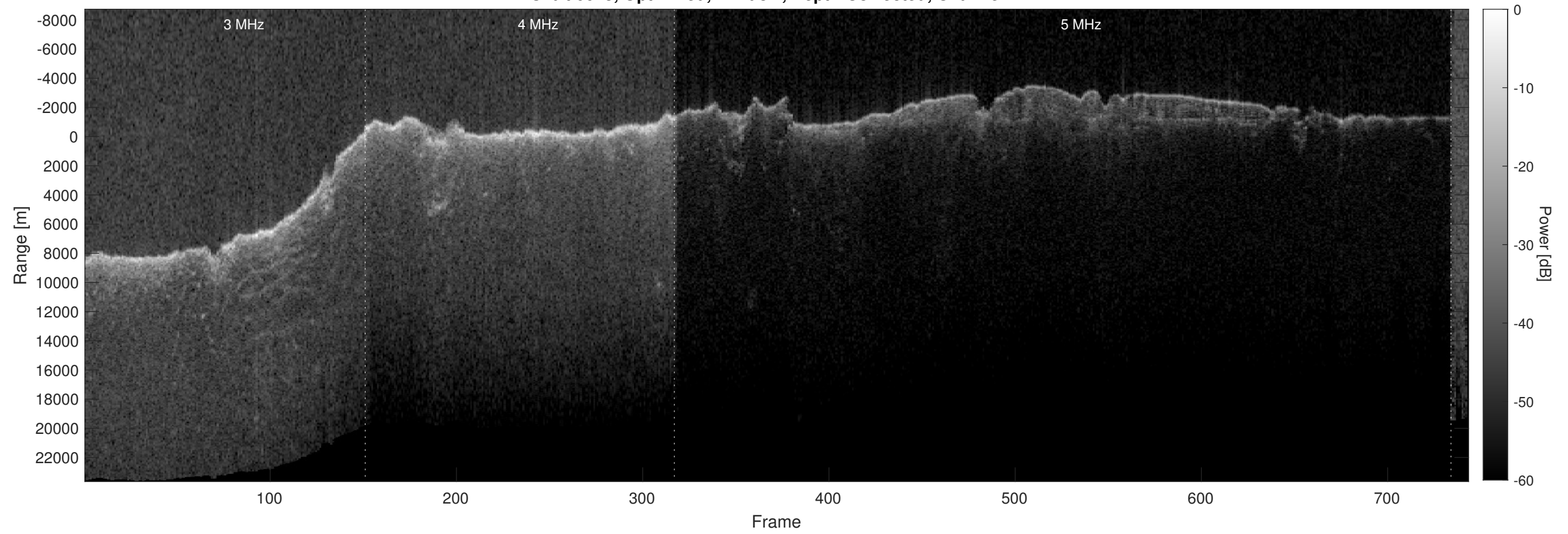
Orbit 6643, Optimized, Window, Depth-Corrected, Channel 2
