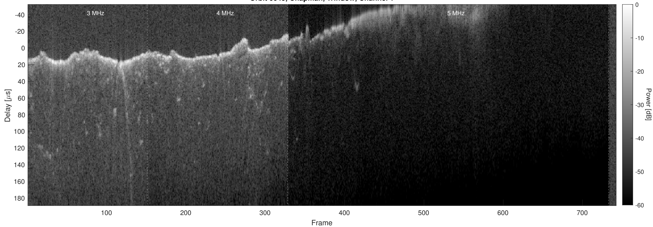
Orbit 6645, Chapman, Window, Channel 2
