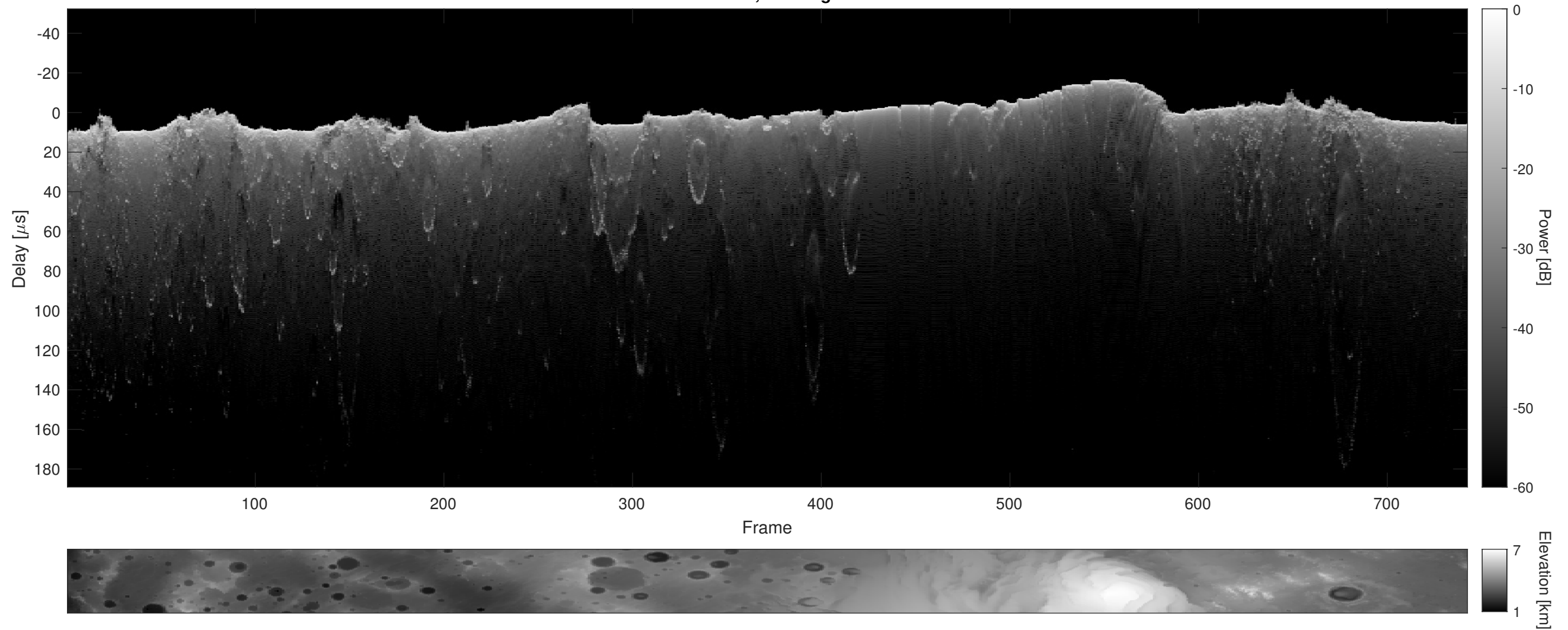
Orbit 6645, Cluttergram
