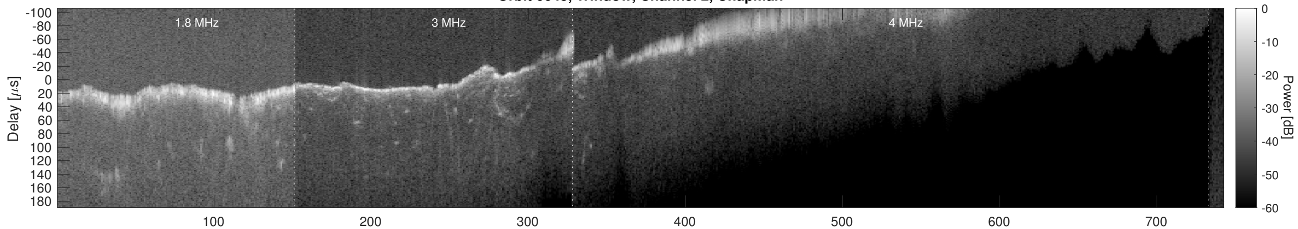
Orbit 6645, Window, Channel 2, Optimized
