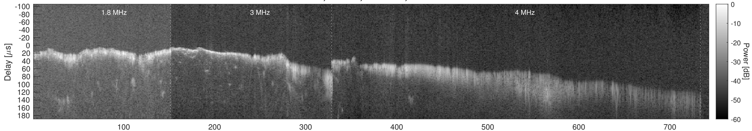
Orbit 6645, Window, Channel 2, Chapman
