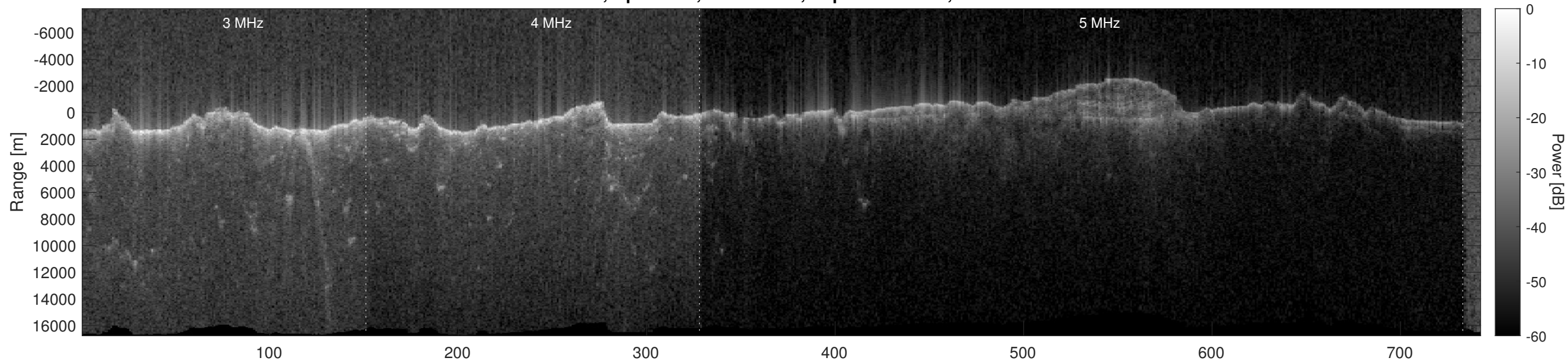
Orbit 6645, Optimized, No Window, Depth-Corrected, Channel 2
