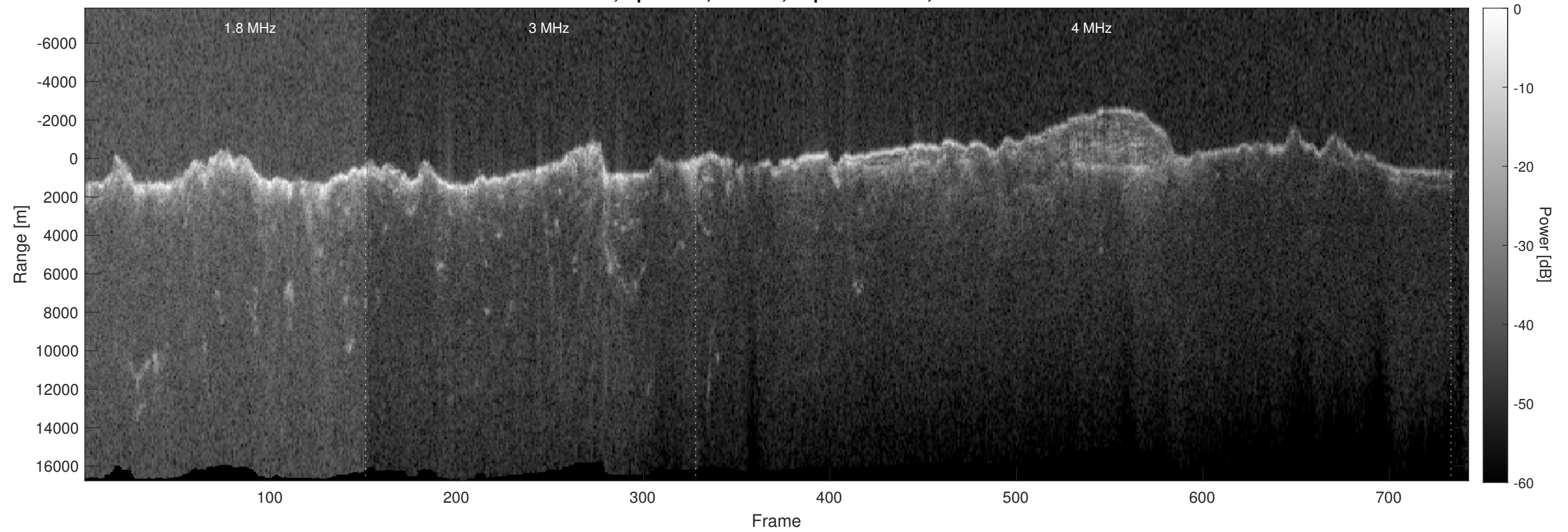
Orbit 6645, Optimized, Window, Depth-Corrected, Channel 2
