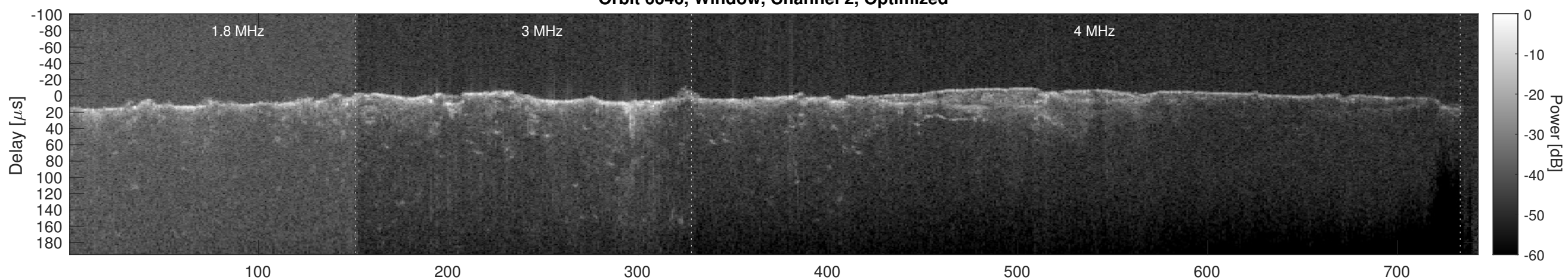
Orbit 6646, Cluttergram
