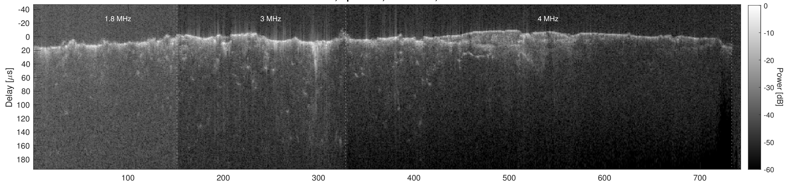
Orbit 6646, Cluttergram
