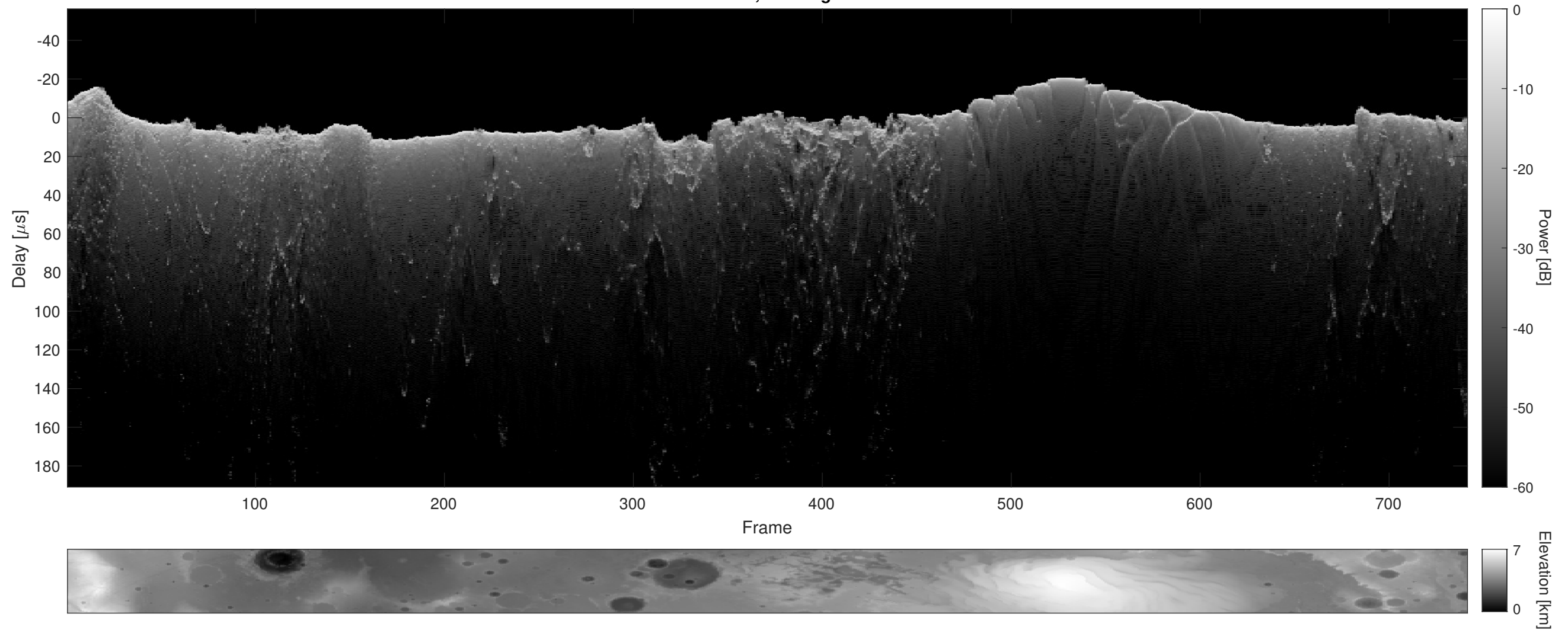
Orbit 6648, Cluttergram
