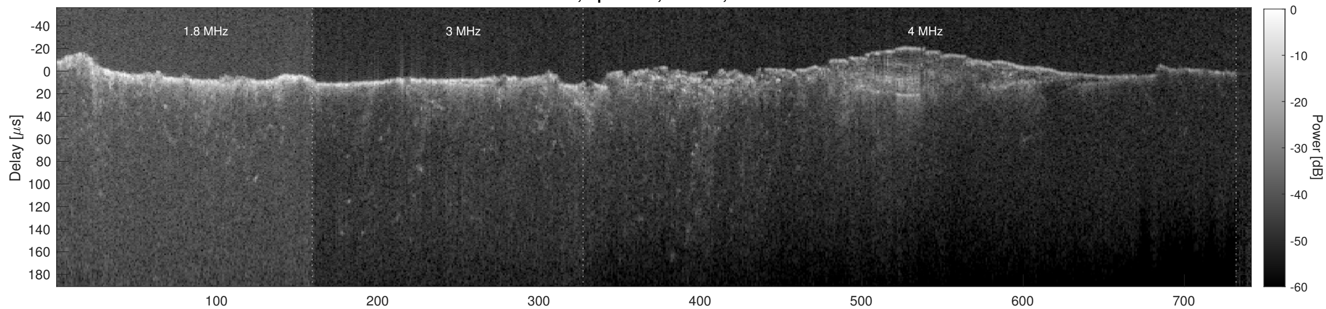
Orbit 6648, Cluttergram
