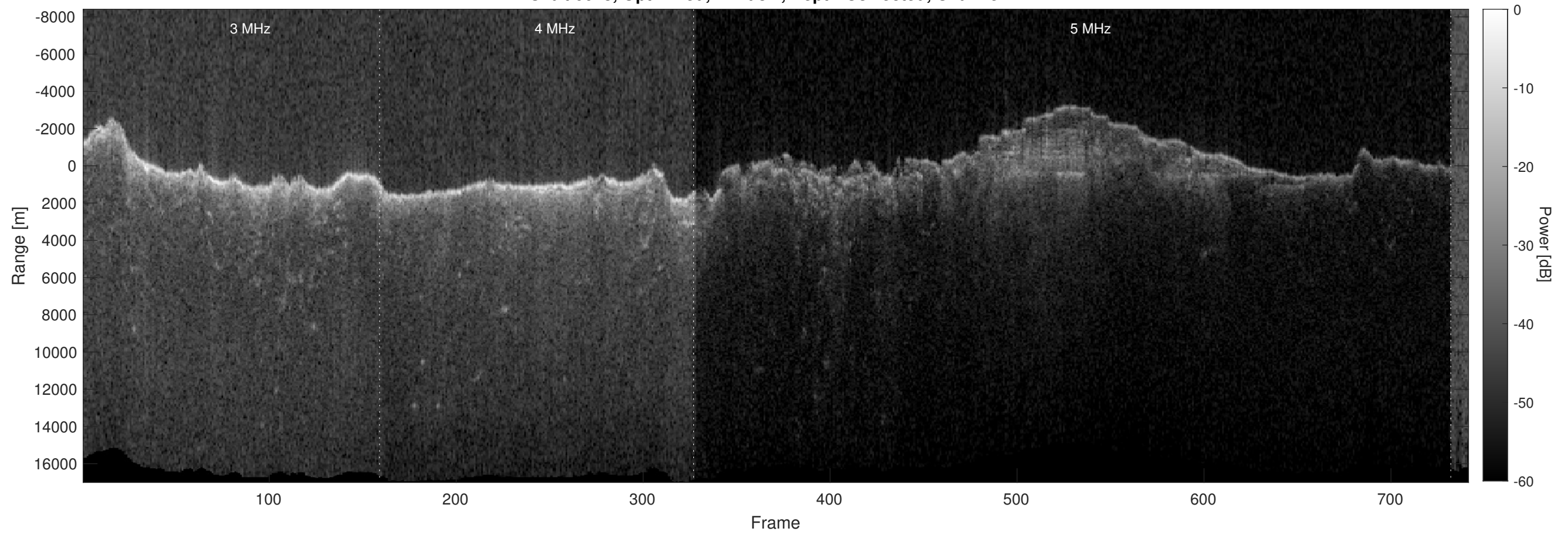
Orbit 6648, Optimized, Window, Depth-Corrected, Channel 2
