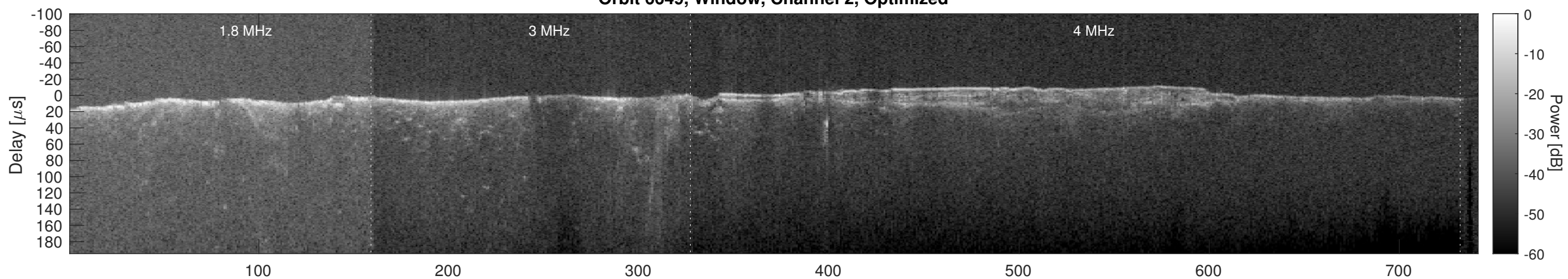
Orbit 6649, Cluttergram
