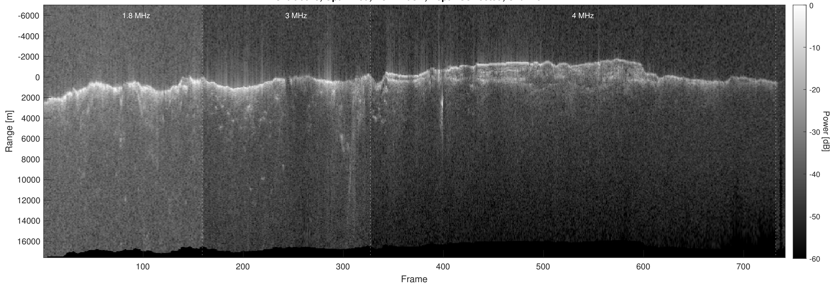
Orbit 6649, Optimized, No Window, Depth-Corrected, Channel 2
