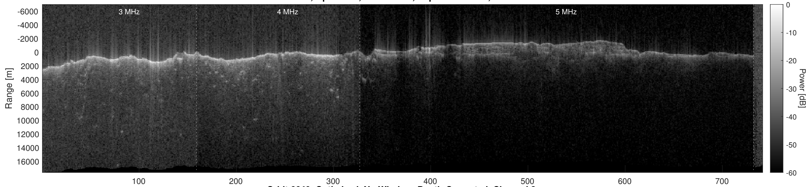
Orbit 6649, Optimized, No Window, Depth-Corrected, Channel 2
