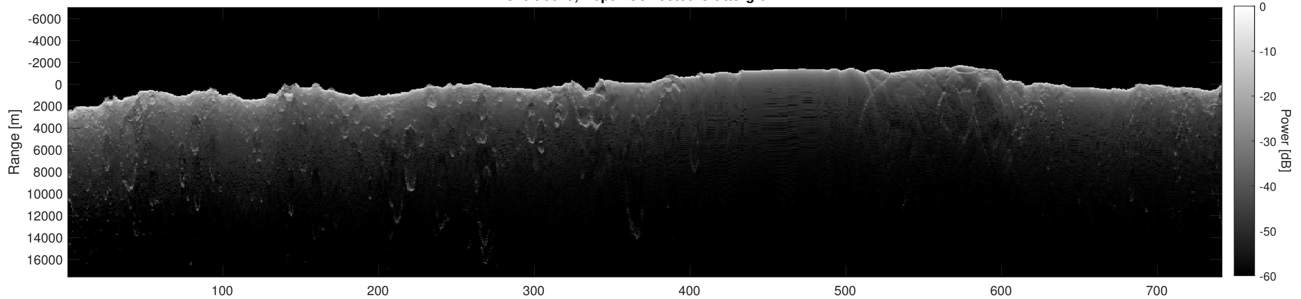
Orbit 6649, Depth-Corrected Cluttergram
