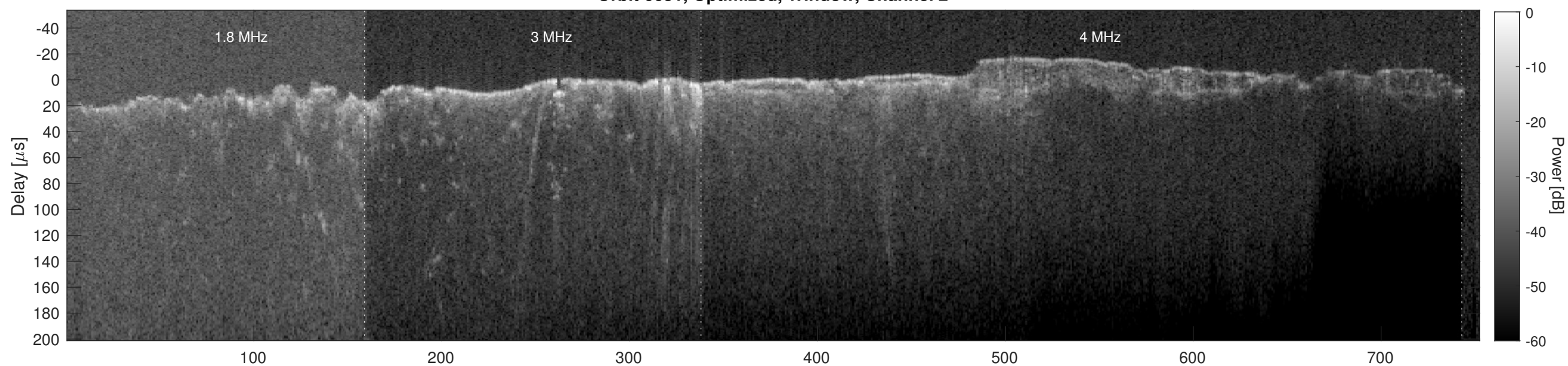
Orbit 6651, Cluttergram
