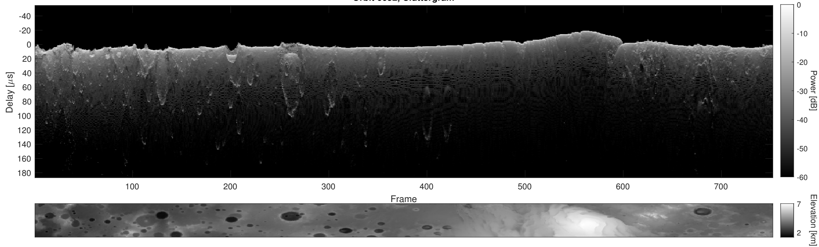
Orbit 6652, Cluttergram
