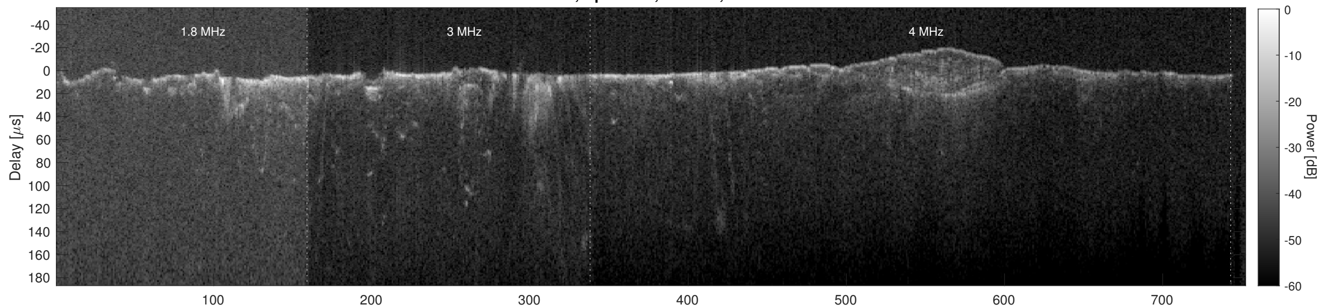
Orbit 6652, Cluttergram
