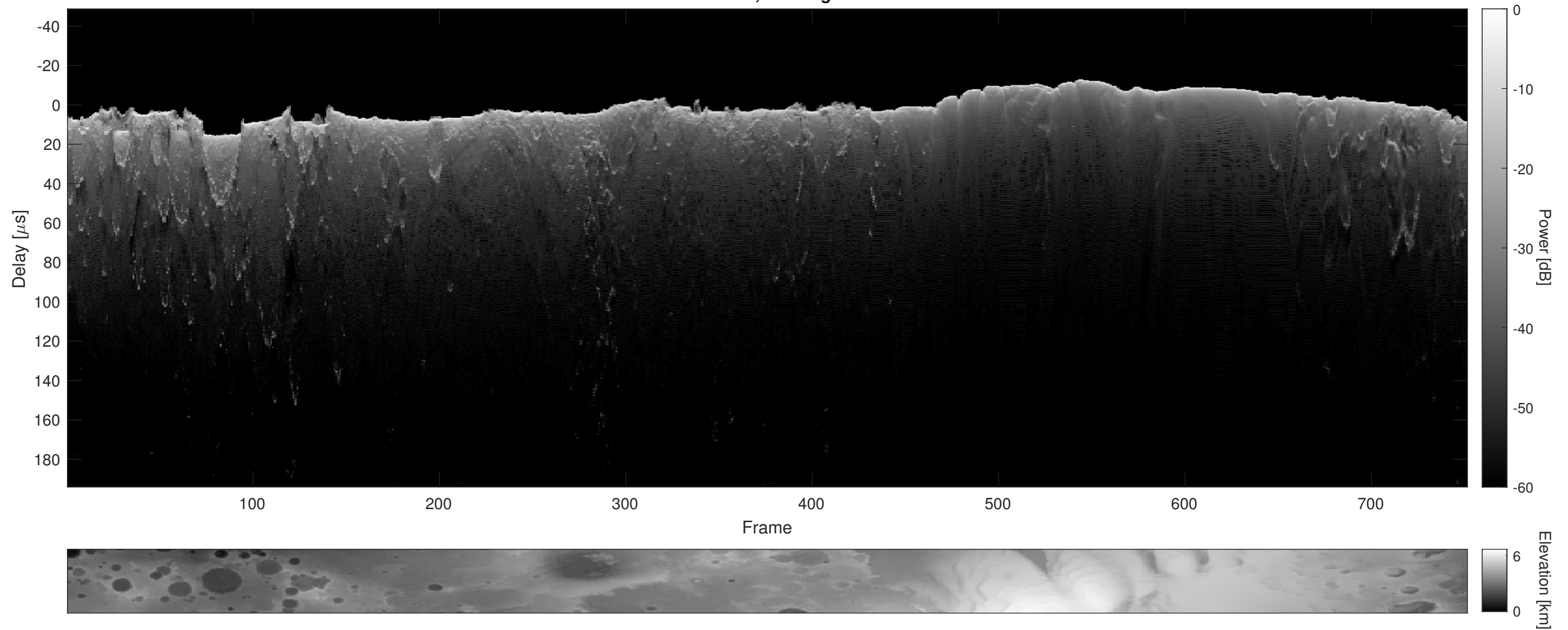
Orbit 6654, Cluttergram
