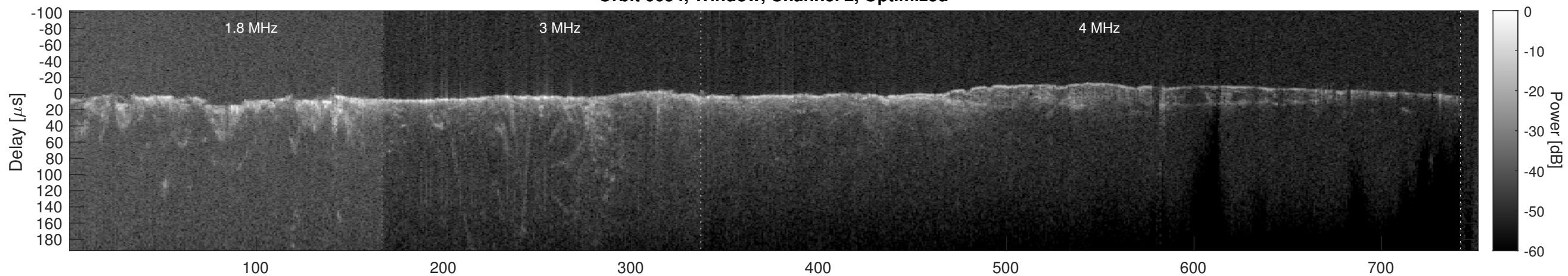
Orbit 6654, Cluttergram
