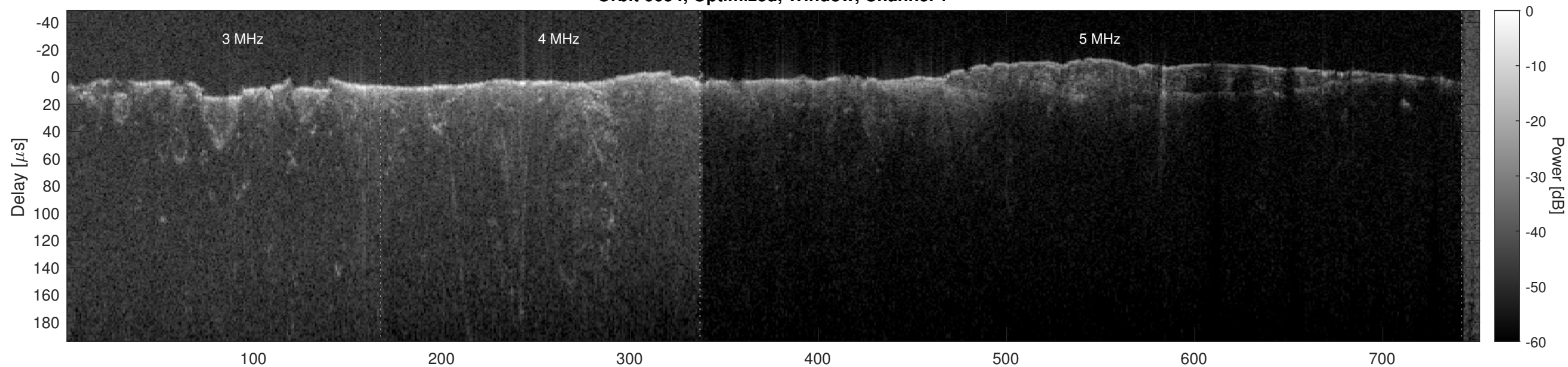
Orbit 6654, Optimized, Window, Channel 2
