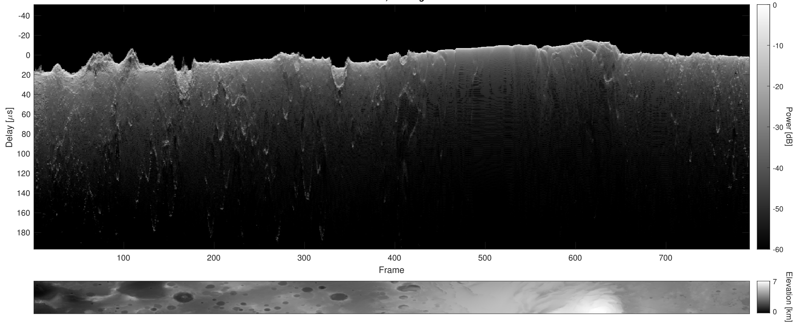
Orbit 6656, Cluttergram
