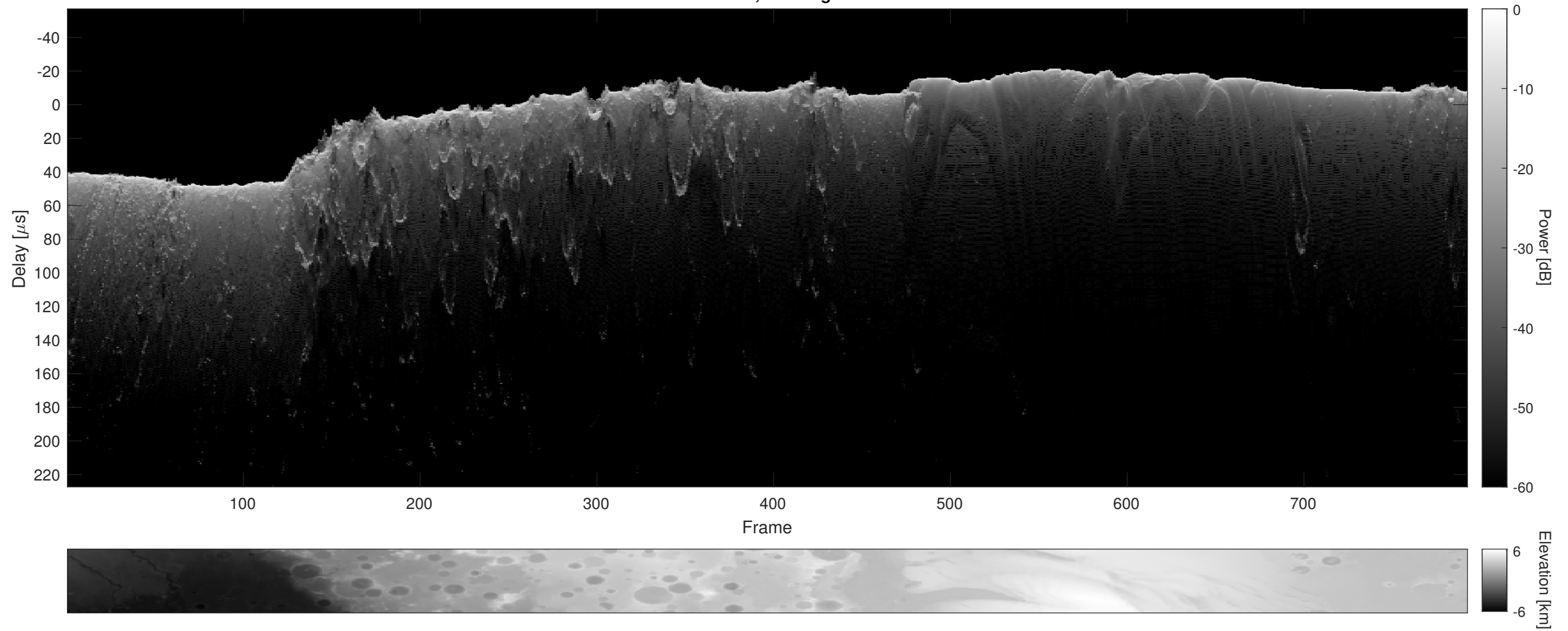
Orbit 6657, Cluttergram
