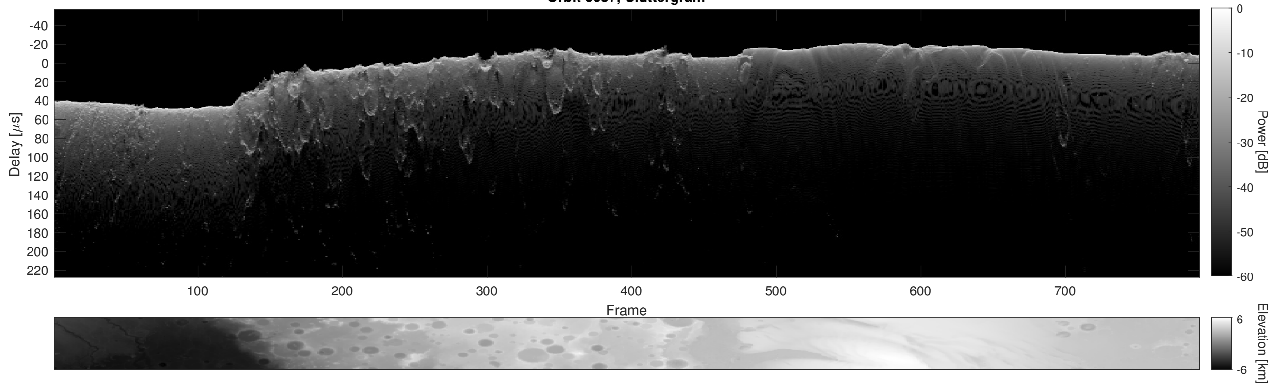
Orbit 6657, Cluttergram
