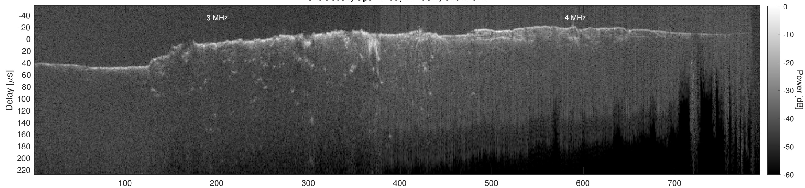
Orbit 6657, Cluttergram
