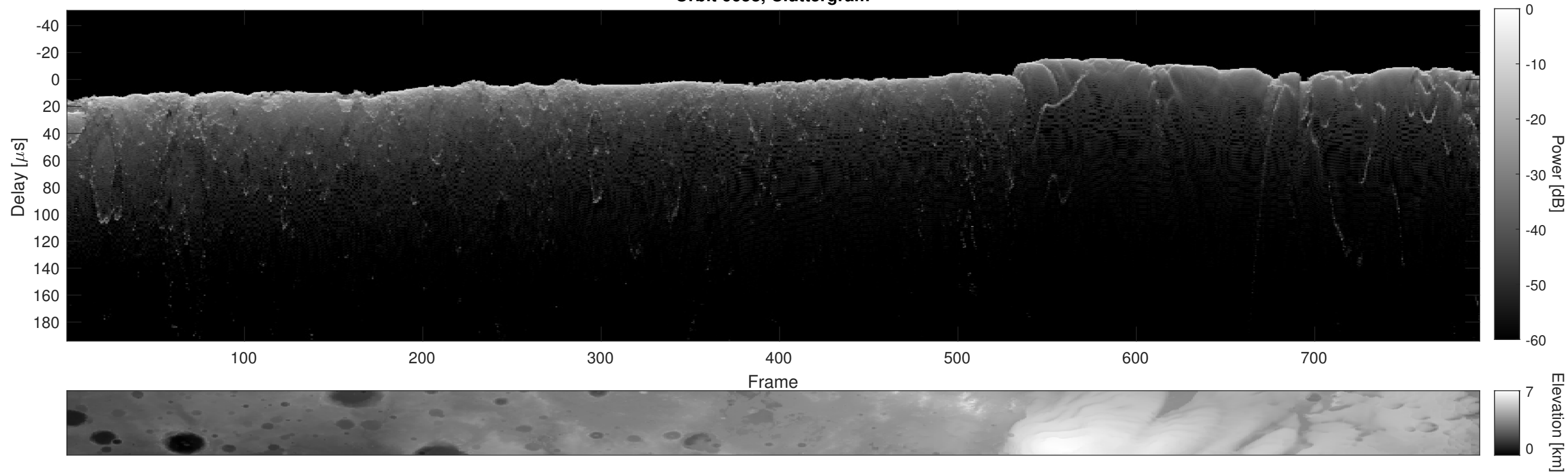
Orbit 6658, Cluttergram
