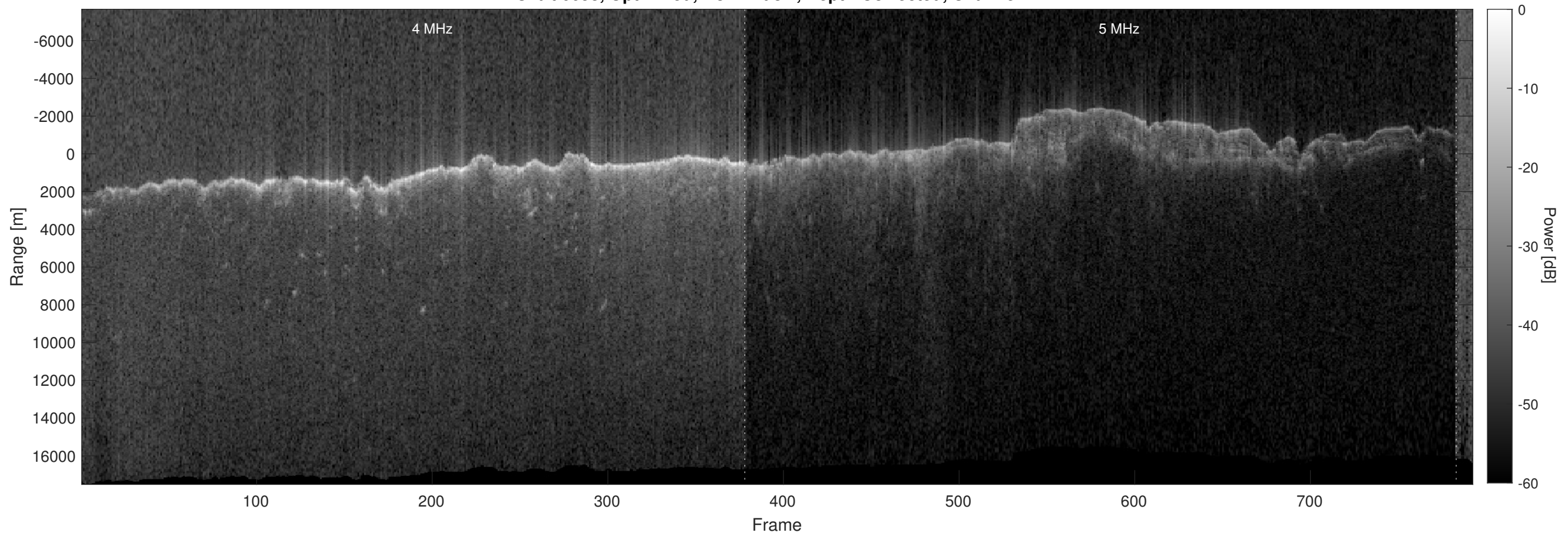
Orbit 6658, Optimized, No Window, Depth-Corrected, Channel 2
