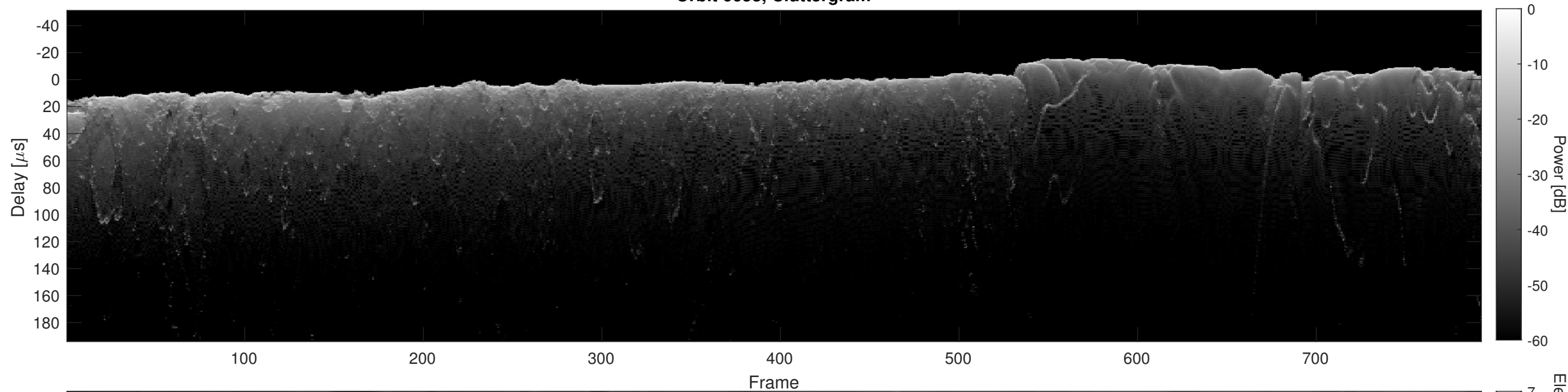
Orbit 6658, Cluttergram
