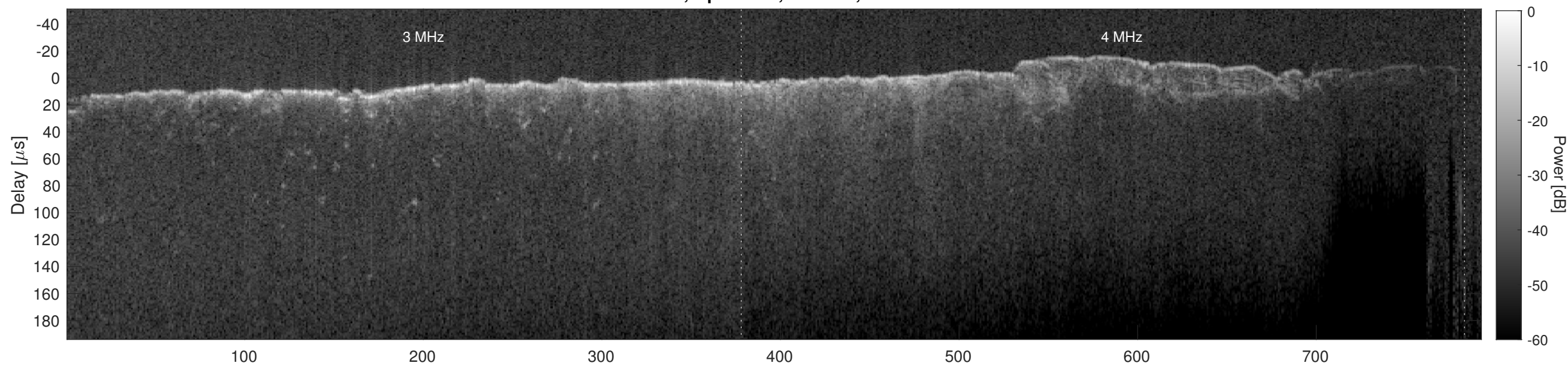
Orbit 6658, Cluttergram
