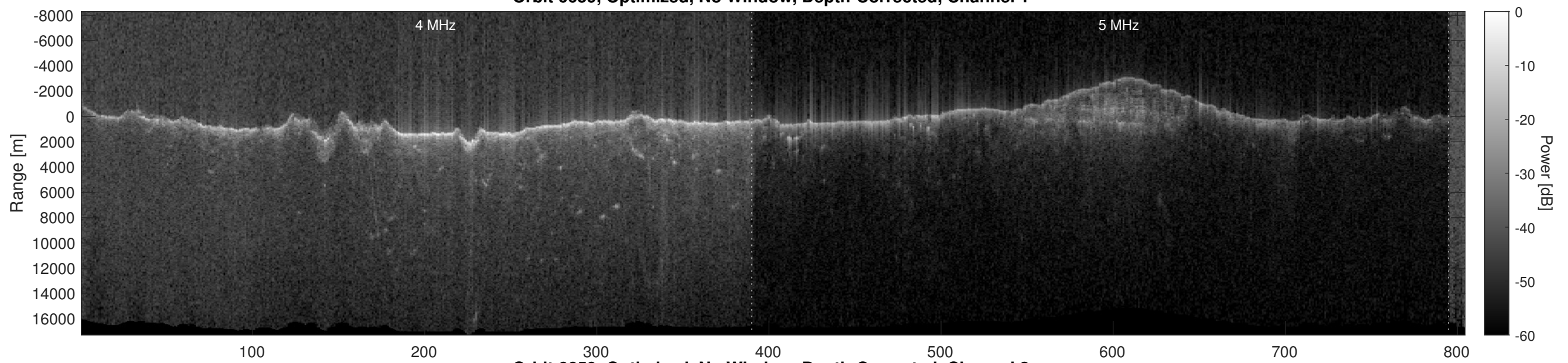
Orbit 6659, Optimized, No Window, Depth-Corrected, Channel 2
