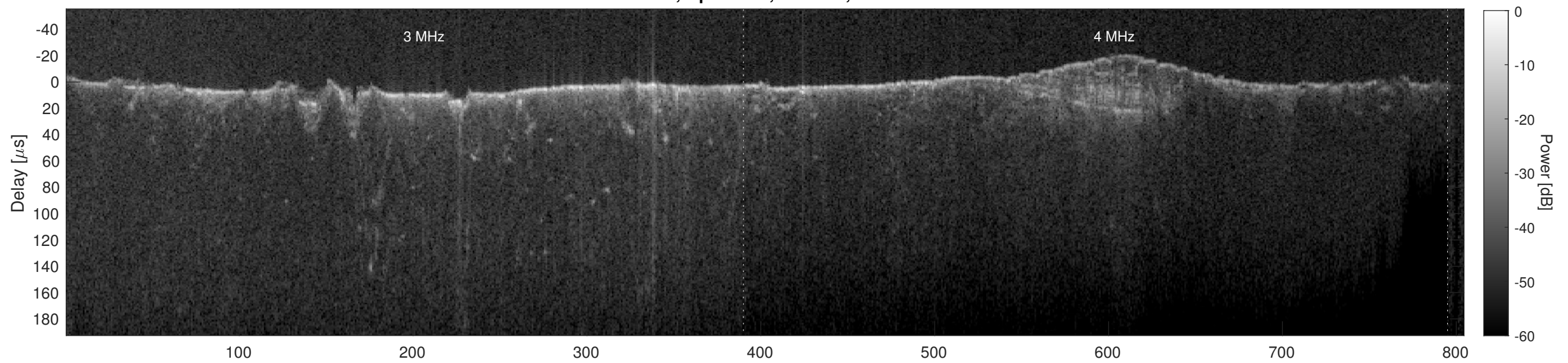
Orbit 6659, Cluttergram
