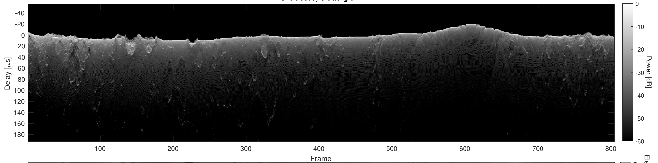
Orbit 6659, Cluttergram
