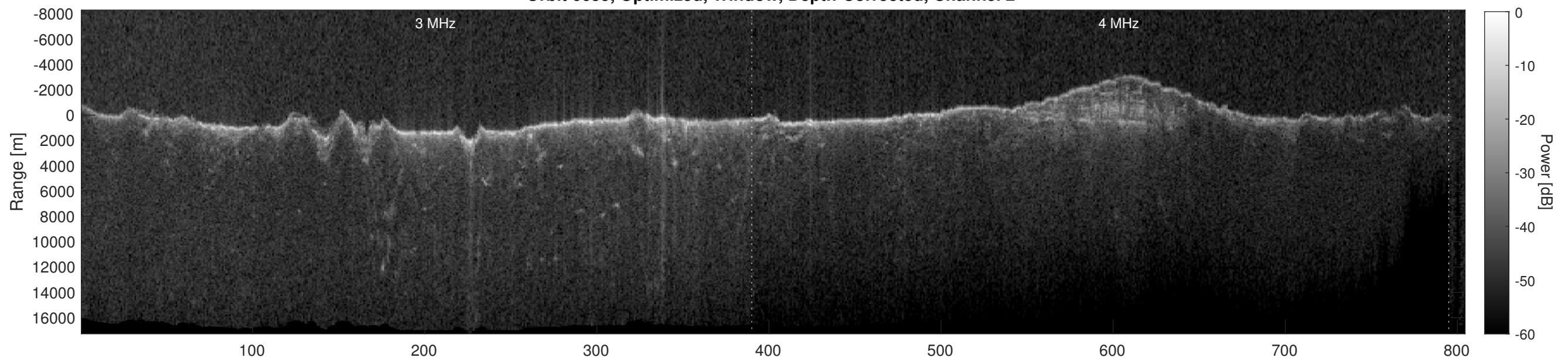
Orbit 6659, Depth-Corrected Cluttergram
