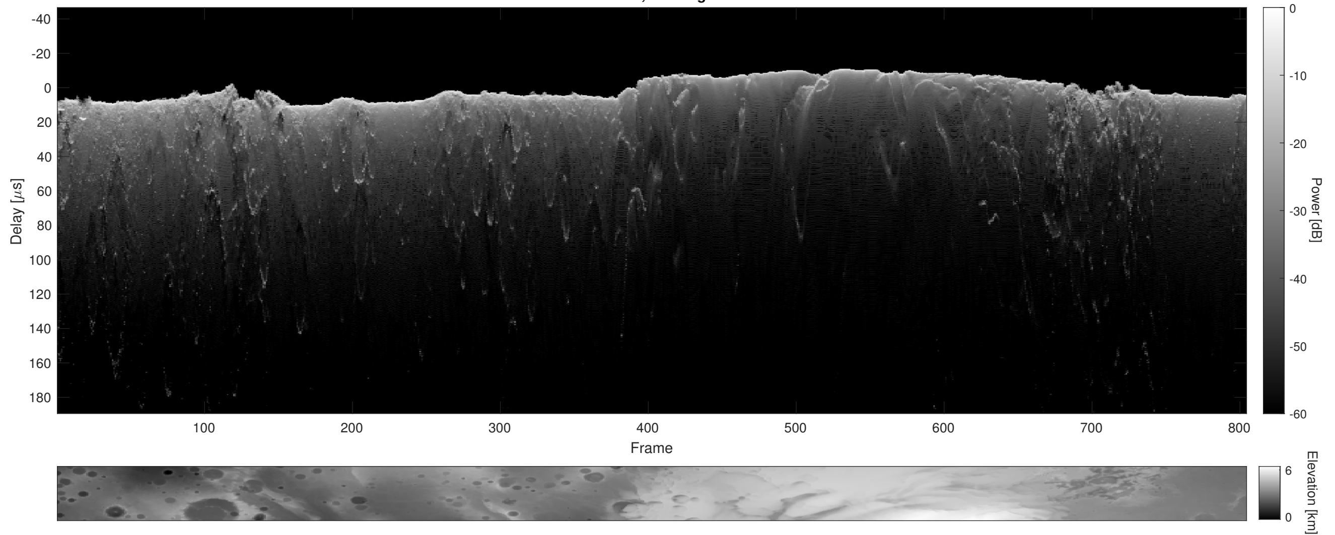
Orbit 6660, Cluttergram
