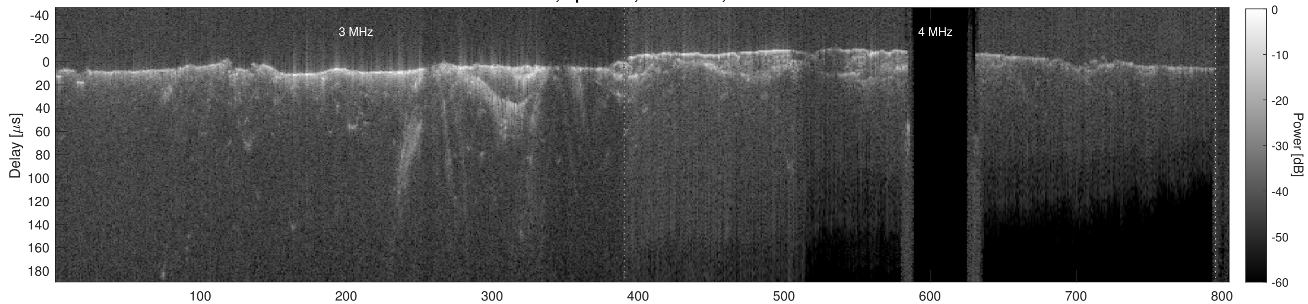
Orbit 6660, Cluttergram
