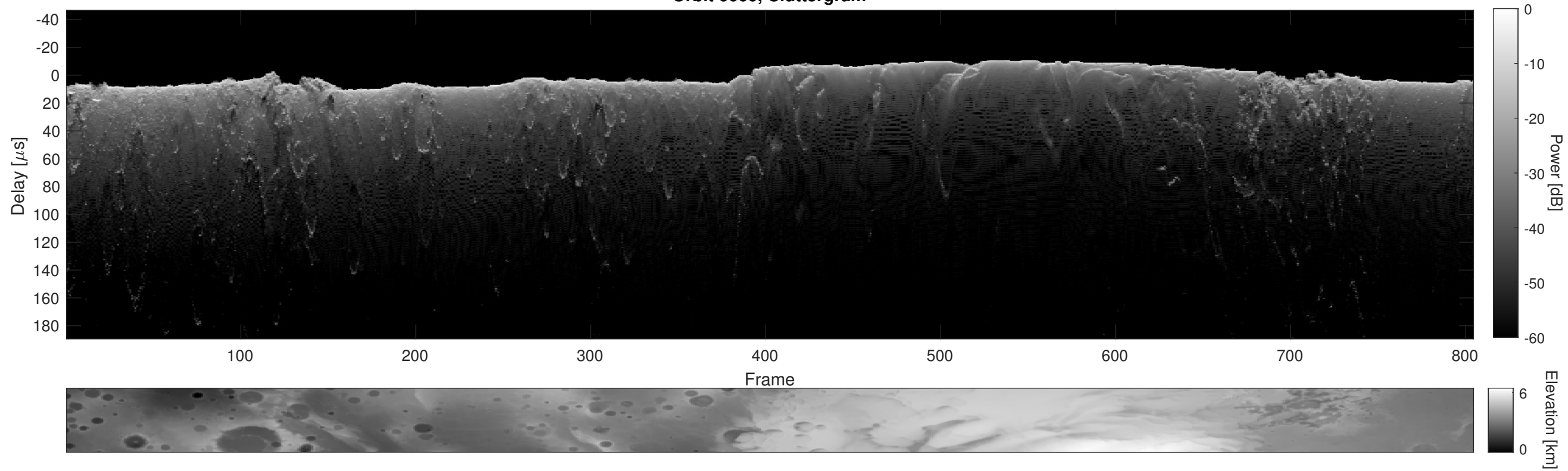
Orbit 6660, Cluttergram
